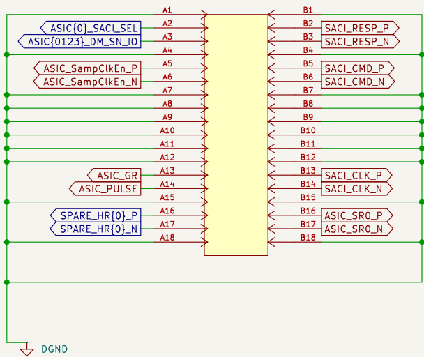
J3 CONN_MINI_SAS_RCPT_36POS_SLD_SMD 757840140:CONN36_B4-0140_MOL
