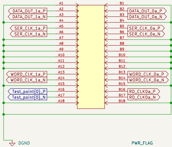
J2 CONN_MINI_SAS_RCPT_36POS_SLD_SMD 757840140:CONN36_B4-0140_MOL
