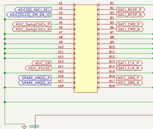
J4 CONN_MINI_SAS_RCPT_36POS_SLD_SMD 757840140:CONN36_B4-0140_MOL
