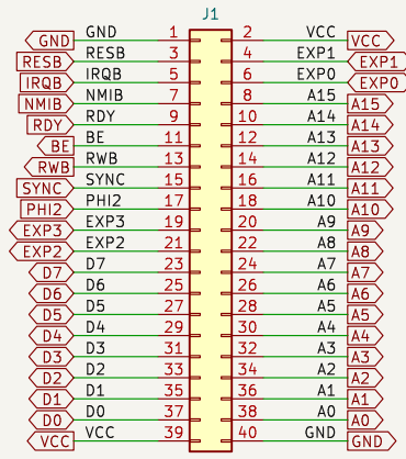
6502 Bus
