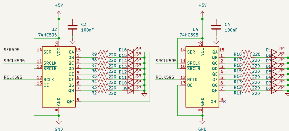
74HC595
