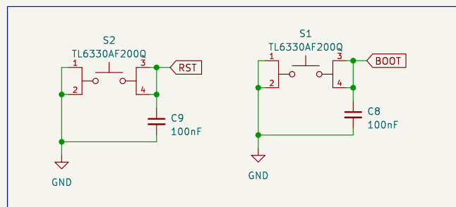
Programming buttons
