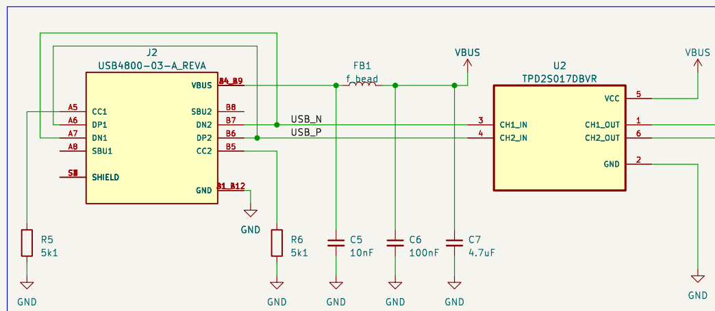
USB connector and ESD protection
