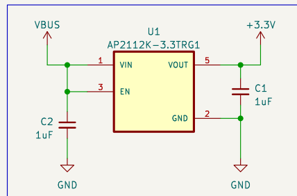
3.3v power
