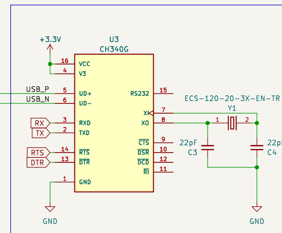
USB to UART
