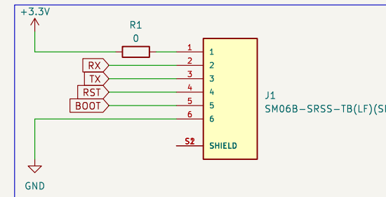
Programming interface
