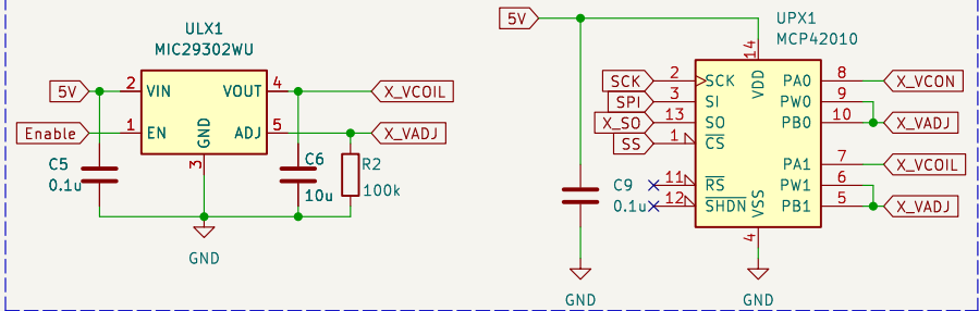
Current Control Circuit
