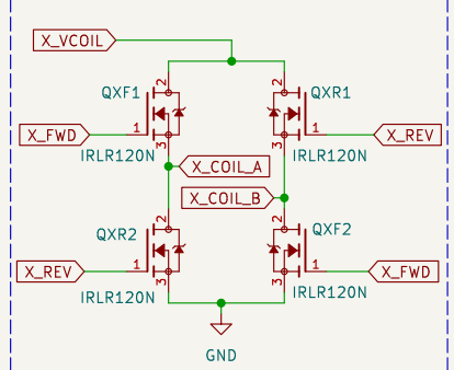
H-Bridge and Coil Connection Circuit
