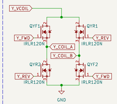
H-Bridge and Coil Connection Circuit
