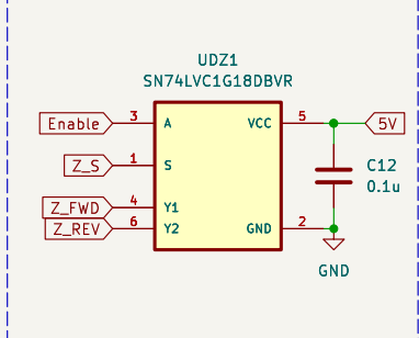
Gate Logic and Amplification Circuit
