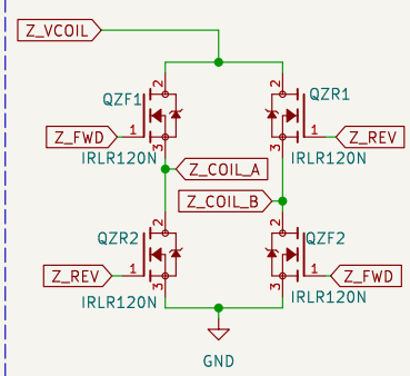
H-Bridge and Coil Connection Circuit
