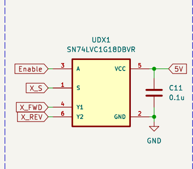
Gate Logic and Amplification Circuit
