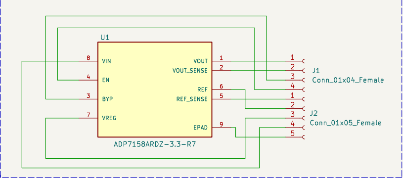
LDO Regulator with 8-SOIC Footprint
