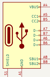
J2 USB_C_Receptacle_USB2.0
